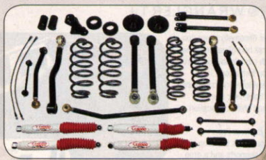
Part No. 44002
